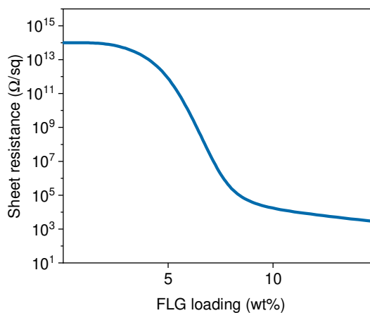
Sheet resistance measured for 40 μm-thick thermoplastic acrylic films as a function of the loading of G-LEAF FLG relative to the dry coating/film weight.
