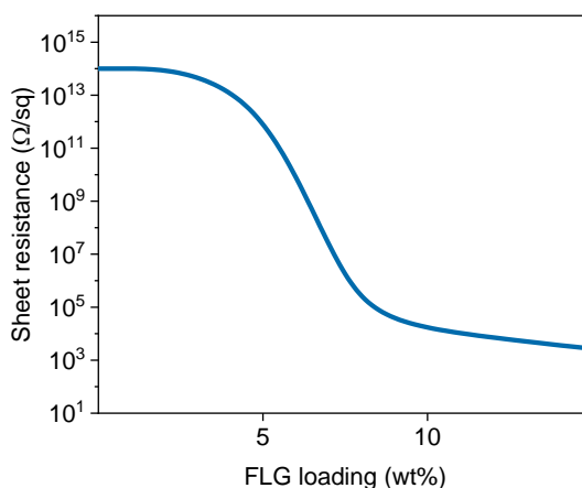
Sheet resistance measured for 40 μm-thick thermoplastic acrylic film as a function of the loading of G-LEAF FLG relative to the dry coating/film weight.
